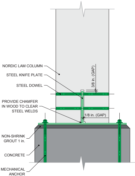
Structure, Base Plate Base Plate with Knife Plate and Four Mechanical Anchors NS-DS2038
