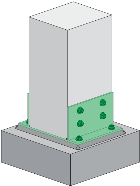
Structure, Base Plate Base Plate with Steel Square NS-DS2037
