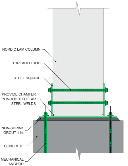
Structure, Base Plate Base Plate with Steel Square NS-DS2037
