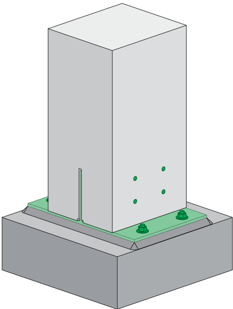
Structure, Base Plate Base Plate with Knife Plate and Four Mechanical Anchors NS-DS2038
