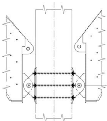
Figure 6: Connecting the arches using pins
