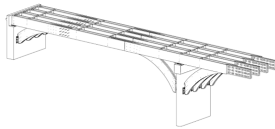
Figure 15: Assembly completed at abutment #5 and pier #4
