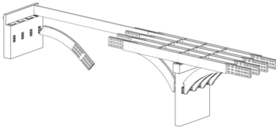
Figure 14: Beginning of assembly at abutment #5
