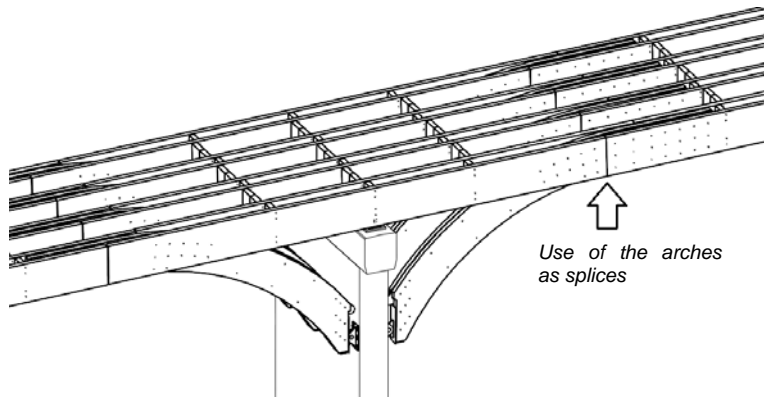
Figure 5: Splicing strategy
