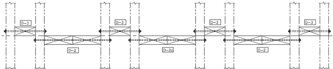
Figure 4: Position of alternate diaphragms
