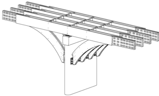
Figure 13: assembly completed at Pier #4
